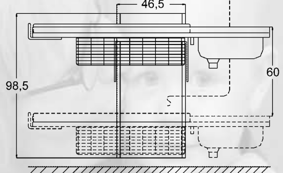
Model 3700 with sink
