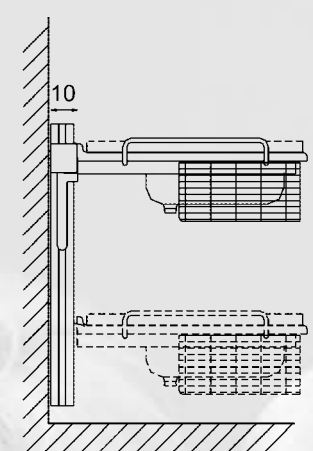
Model 3700 with sink
