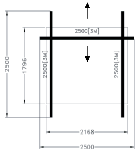
Example 2 : XY System using 2.5m Track (can use any track upto 5m). XY System allows the patient to access all areas within the two parallel tracks
