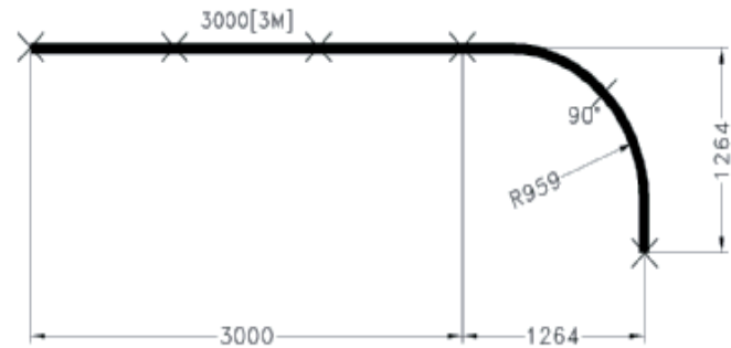
Example 2 : 3m Straight Track with 90 Degree Curve
